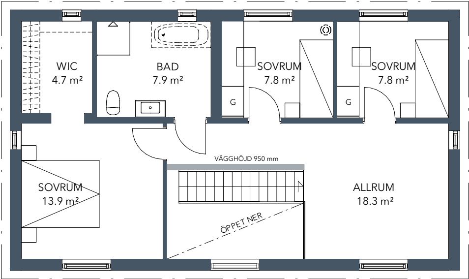
TREND02 plan 2 | Skala 1:100
